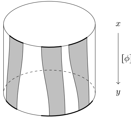
Figure 2: The track of an isotopy representing a 1-cell [\phi]: x \rightarrow y of \mathbf{Mfld}^1/S^1 . X = \mathfrak{s}(x) consists of three copies of the interval [0, 1] , Y = \mathfrak{s}(y) of two. The thick lines at the top and bottom mark the subsets \{0\} \times \text{im } x and \{1\} \times \text{im } y of the cylinder [0, 1] \times S^1 .
