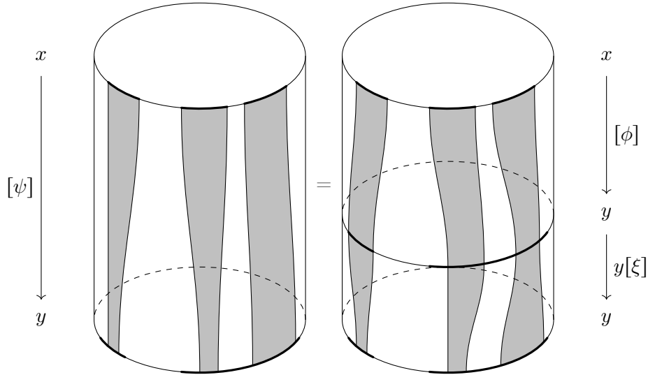
Figure 3: The isotopy \xi: [0, 1] \times X \rightarrow Y between f_\phi and f_\psi represents a 2-cell in (\mathbf{Mfd}^1/S^1)_2([\phi], [\psi]) .
