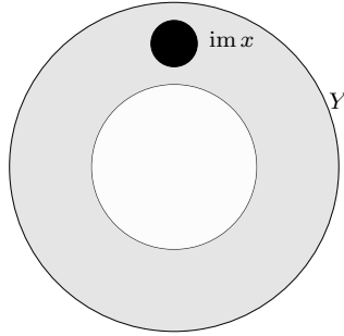
Figure 4: A disc embedded in an annulus
