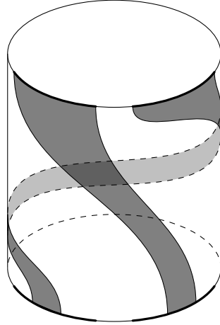
Figure 1: The cyclic operator 1 \rightarrow 1 in \text{ho}(\mathbf{Mfd}^1/S^1) .
